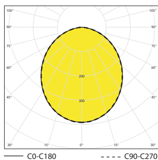
HOOVER-LED-OP-4K, IP65
