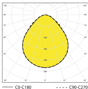
HOOVER-LED-SP-4K, IP65
