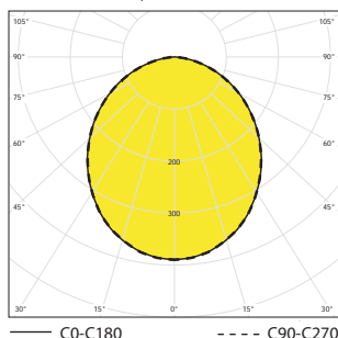
BALOT-LED-OP-4K, IP20/IP40
